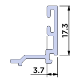
Swing Door Rebate for Adjustable Jamb
