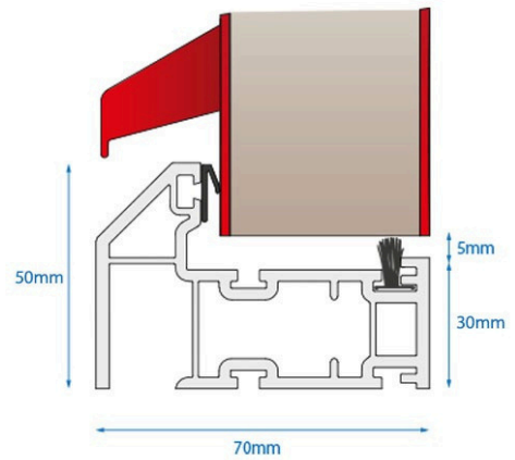
Veka LOW PVC Threshold
