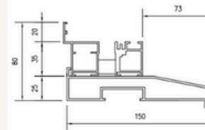
Standard Threshold with 150mm Cill
