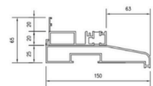
Low Threshold with Rebate & 150mm Cill
