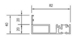
Low Threshold with Rebate - No Cill
