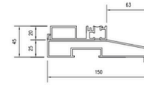
Low Threshold with 150mm Cill
