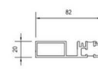
Low Threshold - No Cill
