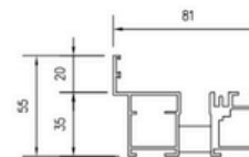
Standard Threshold - No Cill
