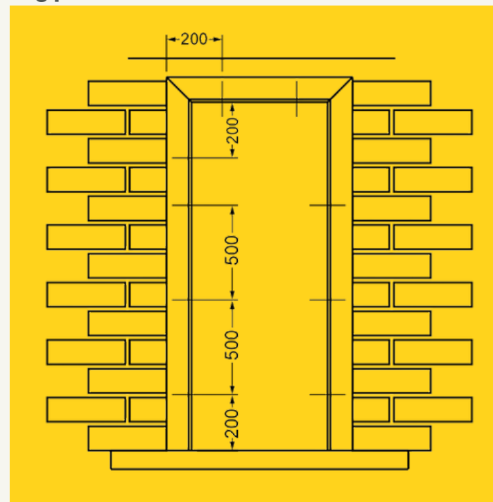
Fig 2: Fixing positions
