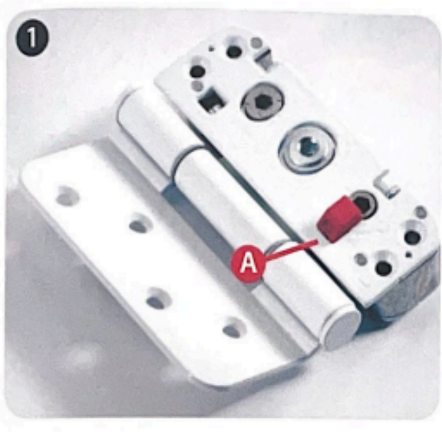
With the door upright pull out and dispose of the red locking wedge (A).
