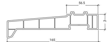
LCL165 165mm Cill
