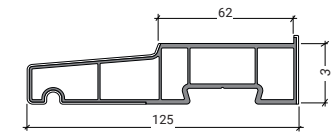
LSL125 125mm Cill
