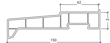
LSL150 150mm Cill
