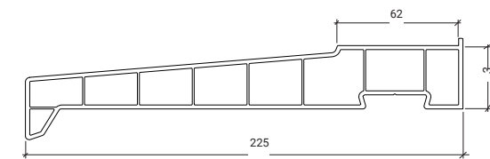
LSL225 225mm Cill
