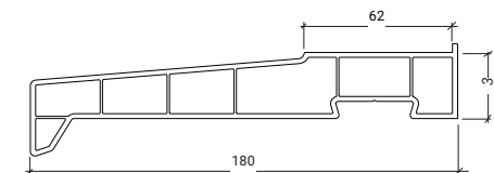
LSL180 180mm Cill
