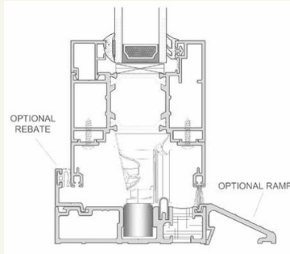
Low threshold detail
