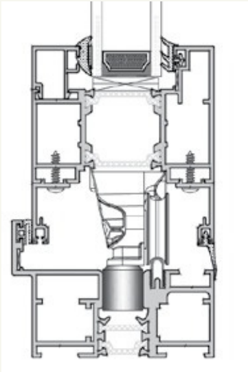
Standard threshold detail
