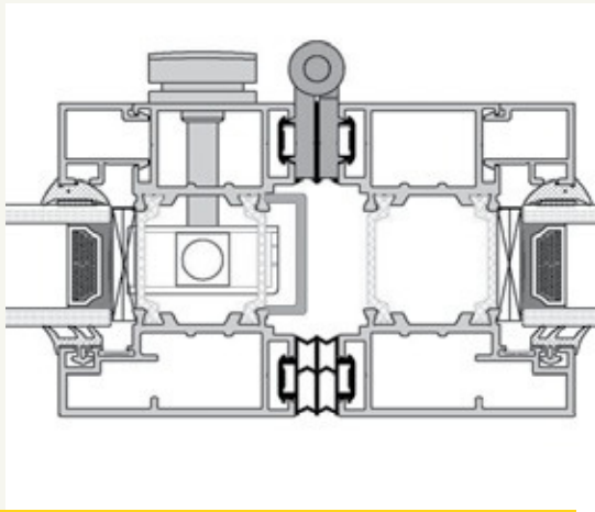
Intermediate detail integrated lock
