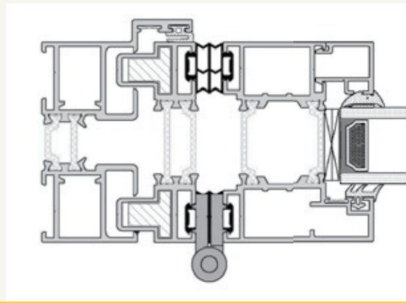
Outer frame detail with adjustable jamba
